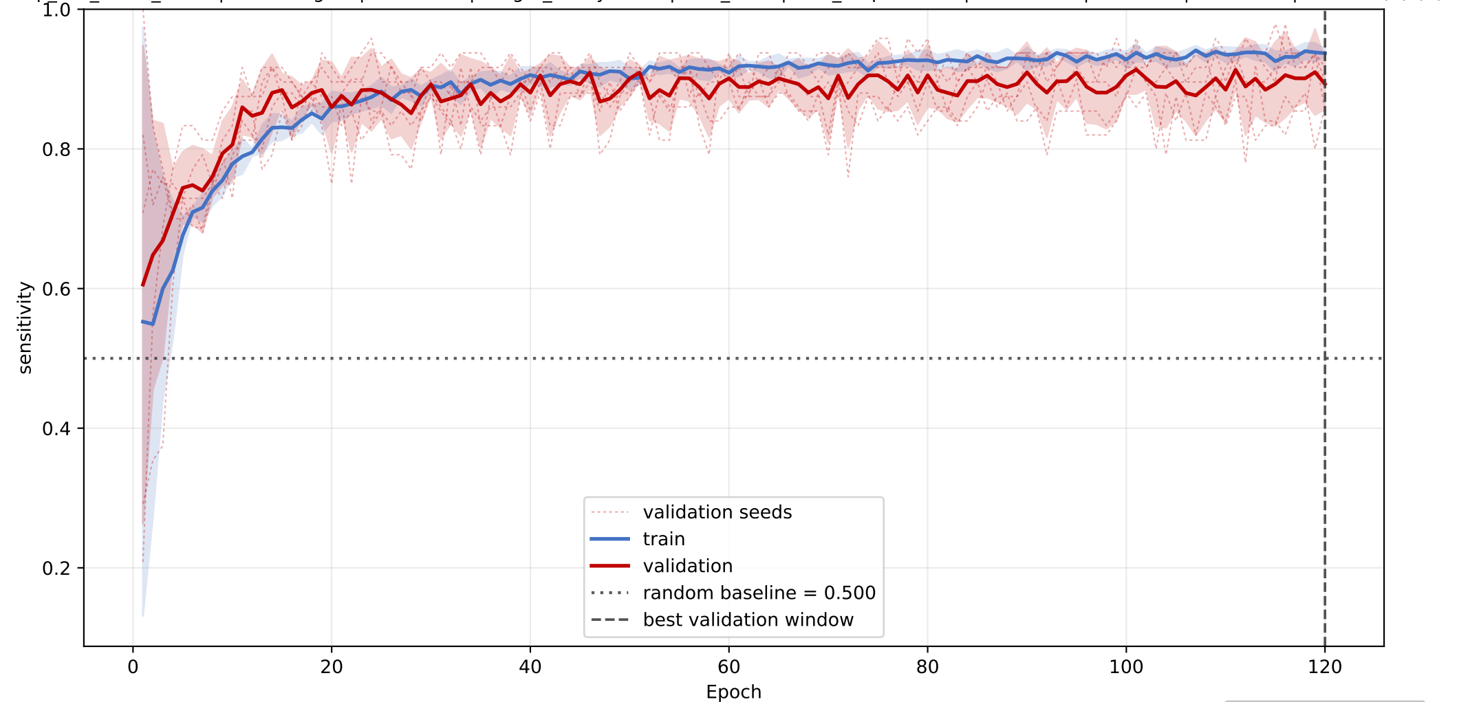
species15: mean sensitivity learning curve across seeds
