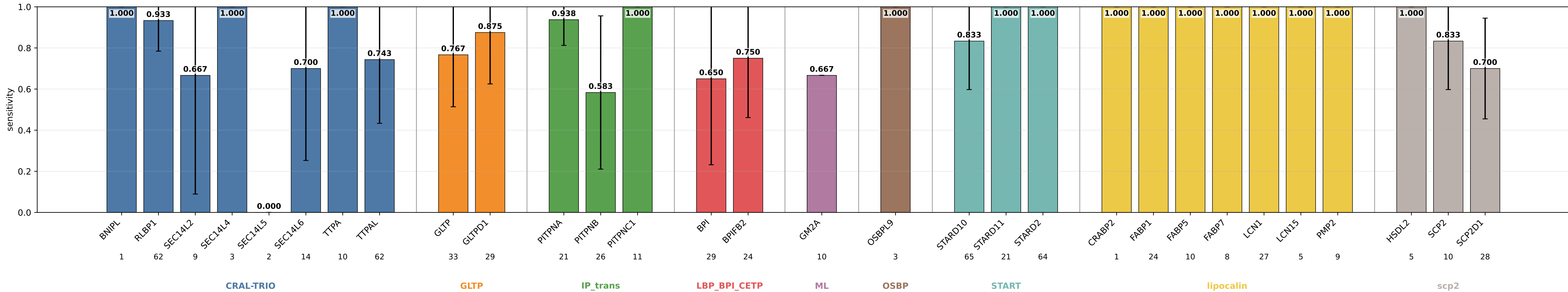
mlp_s15_nomb_hid64 sensitivity by subgroup mlp_s15_nomb_hid64 | class weights | lr=0.0001 | weight_decay=0.01 | final_m=4 | final_dropout=0.1 | hiddim=64 | heads=8 | batch=16 | ep=120 | seeds=0,1,2,3,4
