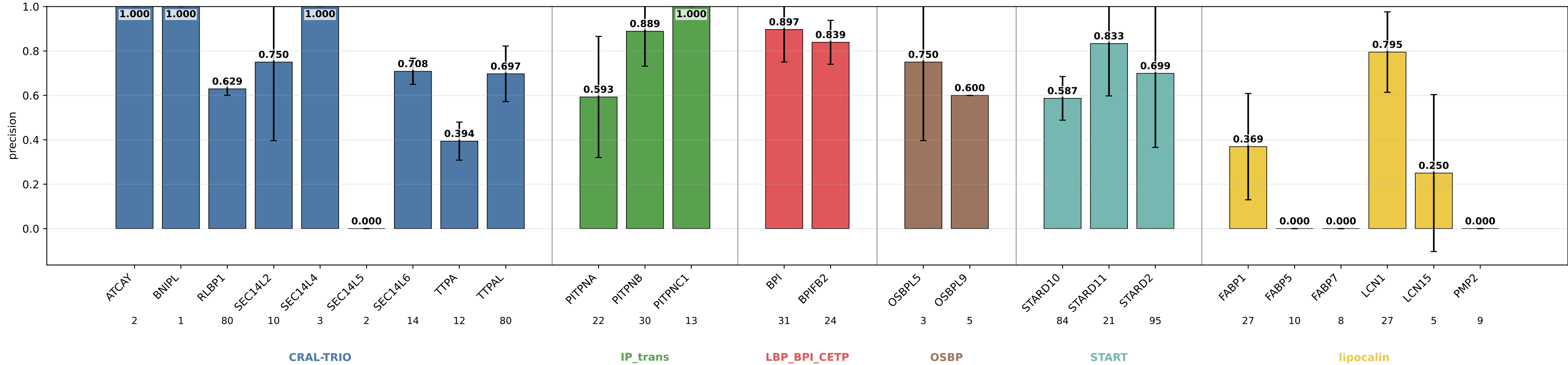
bbp_smd_fa_pockets_only_nps3mlp_dpt01_gm_plm64_hid64_ep120 precision by subgroup bbp_smd_fa_pockets_only_nps3mlp_dpt01_gm_plm64_hid64_ep120 | class weights | lr=0.0001 | weight_decay=0.001 | final_m=4 | final_dropout=0.1 | hiddim=64 | heads=8 | batch=16 | ep=120 | seeds=0,1
