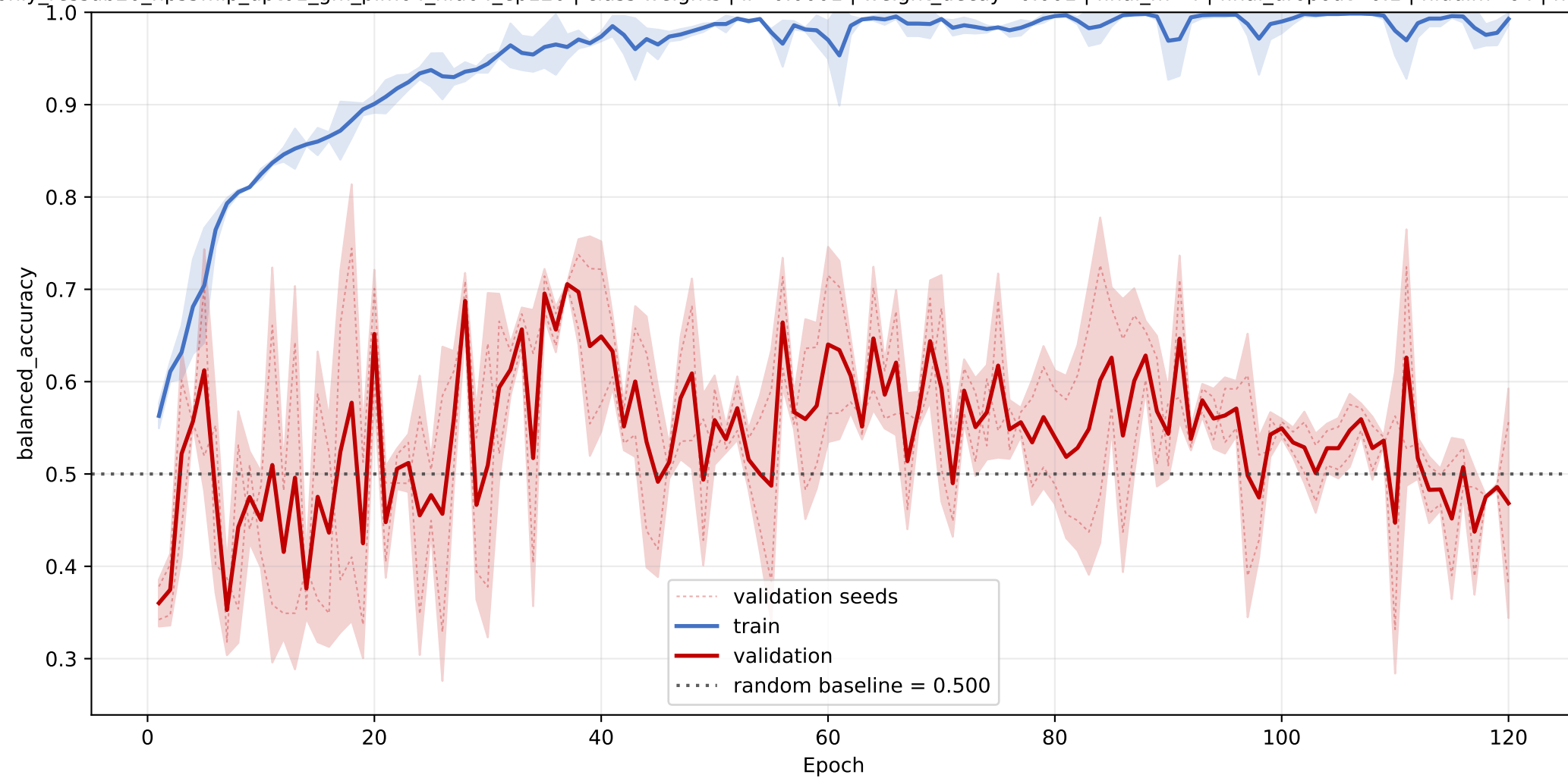
CRAL-TRIO: mean balanced accuracy learning curve across seeds
