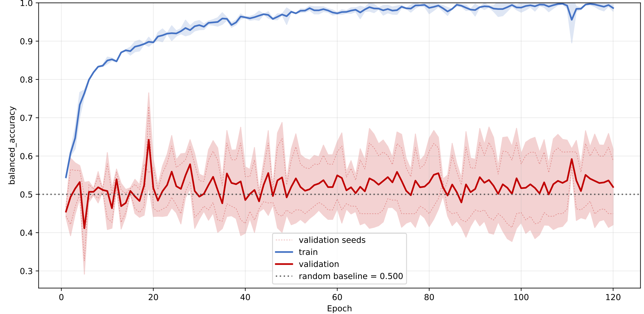
lipocalin: mean balanced_accuracy learning curve across seeds
