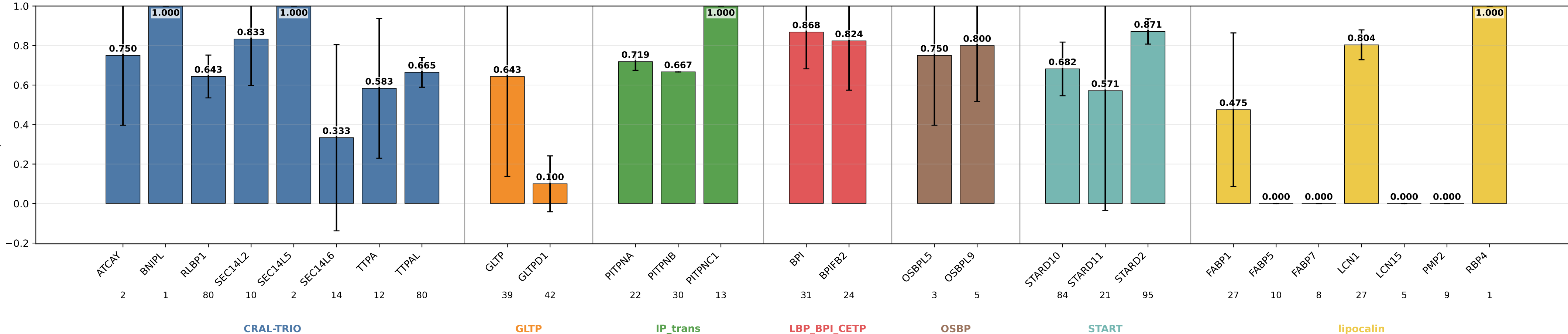
bbp_smd_fa_pockets_only_ressub20_nps3mlp_dpt01_gm_plm64_hid64_ep120 precision by subgroup bbp_smd_fa_pockets_only_ressub20_nps3mlp_dpt01_gm_plm64_hid64_ep120 | class weights | lr=0.0001 | weight_decay=0.001 | final_m=4 | final_dropout=0.1 | hiddim=64 | heads=8 | batch=16 | ep=120 | seeds=0,1
