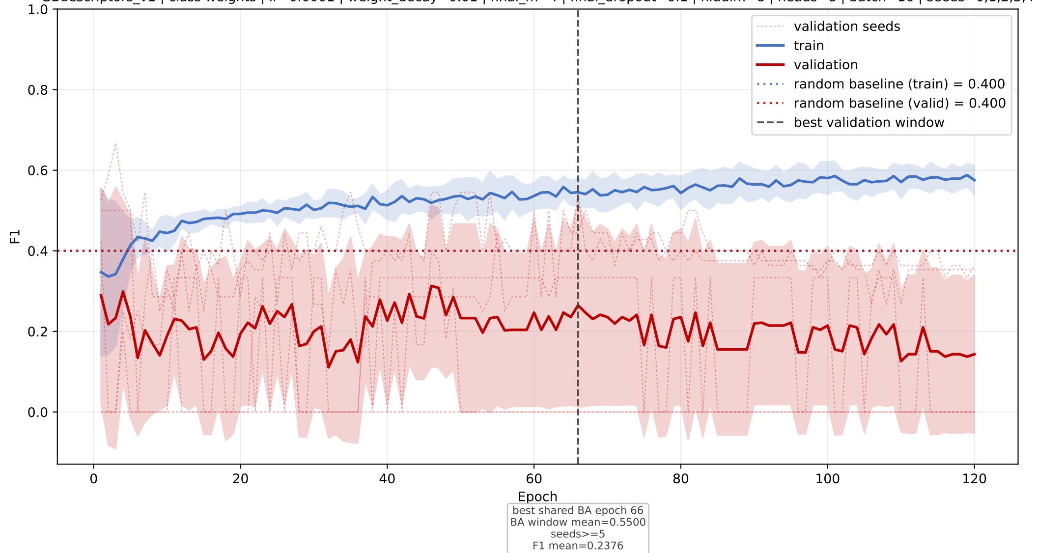
ML: mean F1 learning curve across seeds
