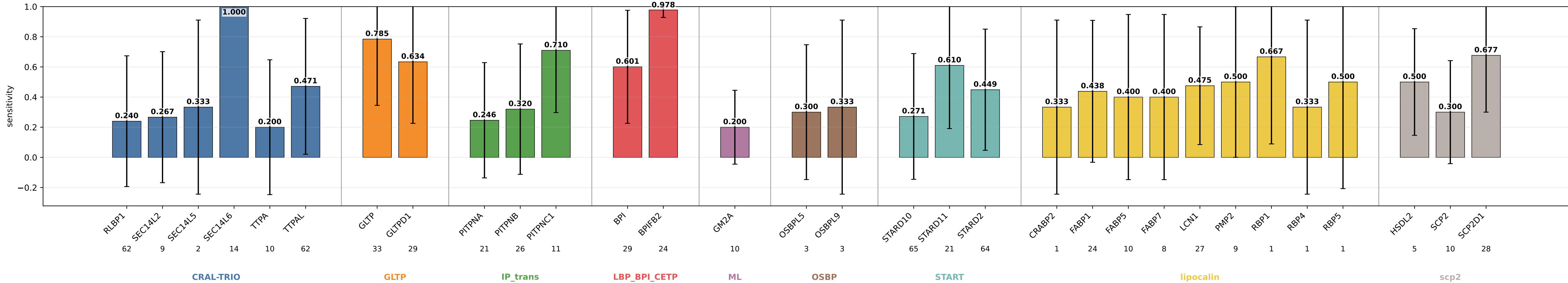
GBdescriptors_v1 sensitivity by subgroup GBdescriptors_v1 | class weights | lr=0.0001 | weight_decay=0.01 | final_m=4 | final_dropout=0.1 | hiddim=8 | heads=8 | batch=16 | ep=120 | seeds=0,1,2,3,4
