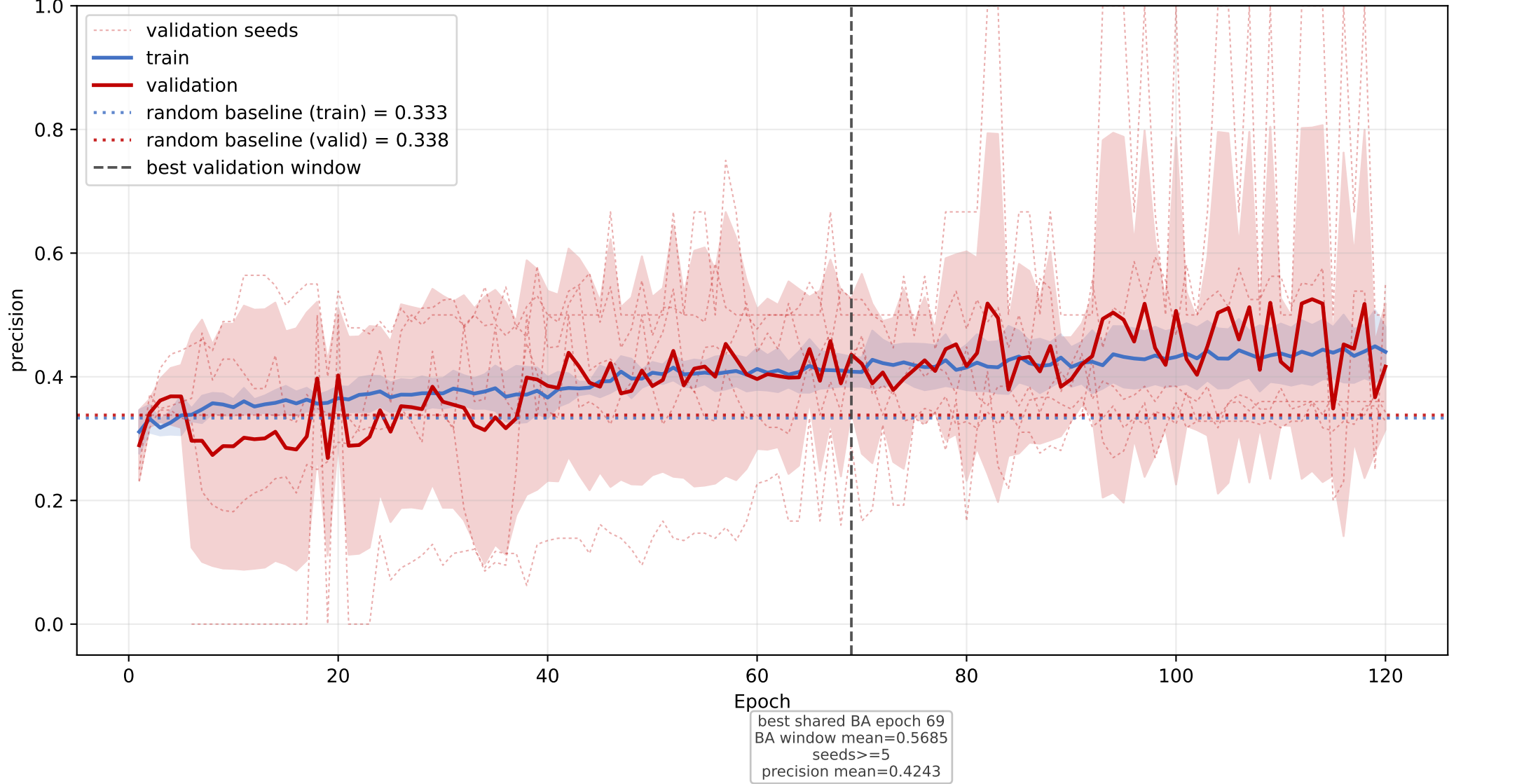
LBP_BPI_CETP: mean precision learning curve across seeds
