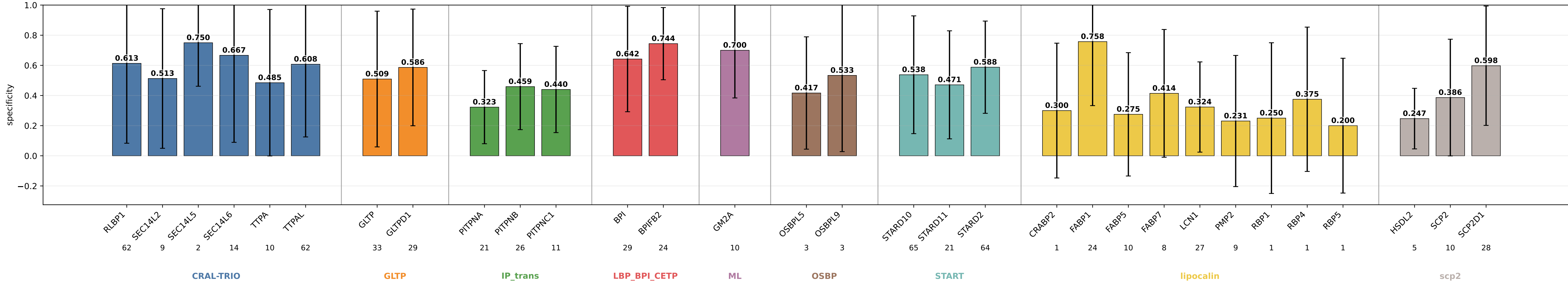
GBdescriptors_v1_depth_bulk_match specificity by subgroup GBdescriptors_v1_depth_bulk_match | class weights | lr=0.0001 | weight_decay=0.01 | final_m=4 | final_dropout=0.1 | hiddim=8 | heads=8 | batch=16 | ep=120 | seeds=0,1,2,3,4
