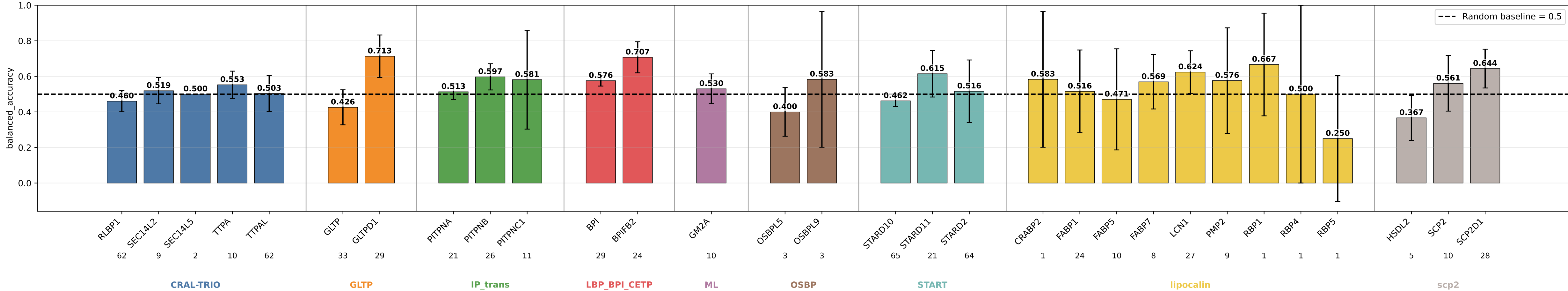
GBdescriptors_v1_ocpnc balanced_accuracy by subgroup GBdescriptors_v1_ocpnc | class weights | lr=0.0001 | weight_decay=0.01 | final_m=4 | final_dropout=0.1 | hiddim=8 | heads=8 | batch=16 | ep=120 | seeds=0,1,2,3,4
