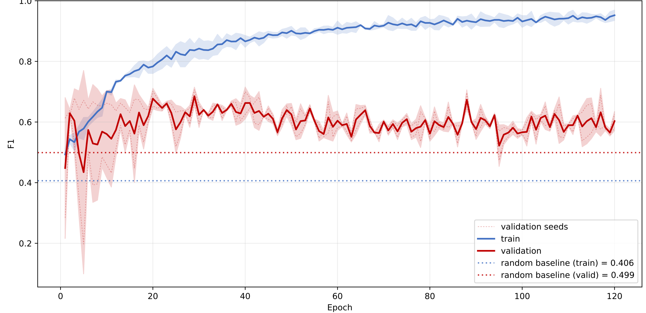
CRAL-TRIO: mean F1 learning curve across seeds
