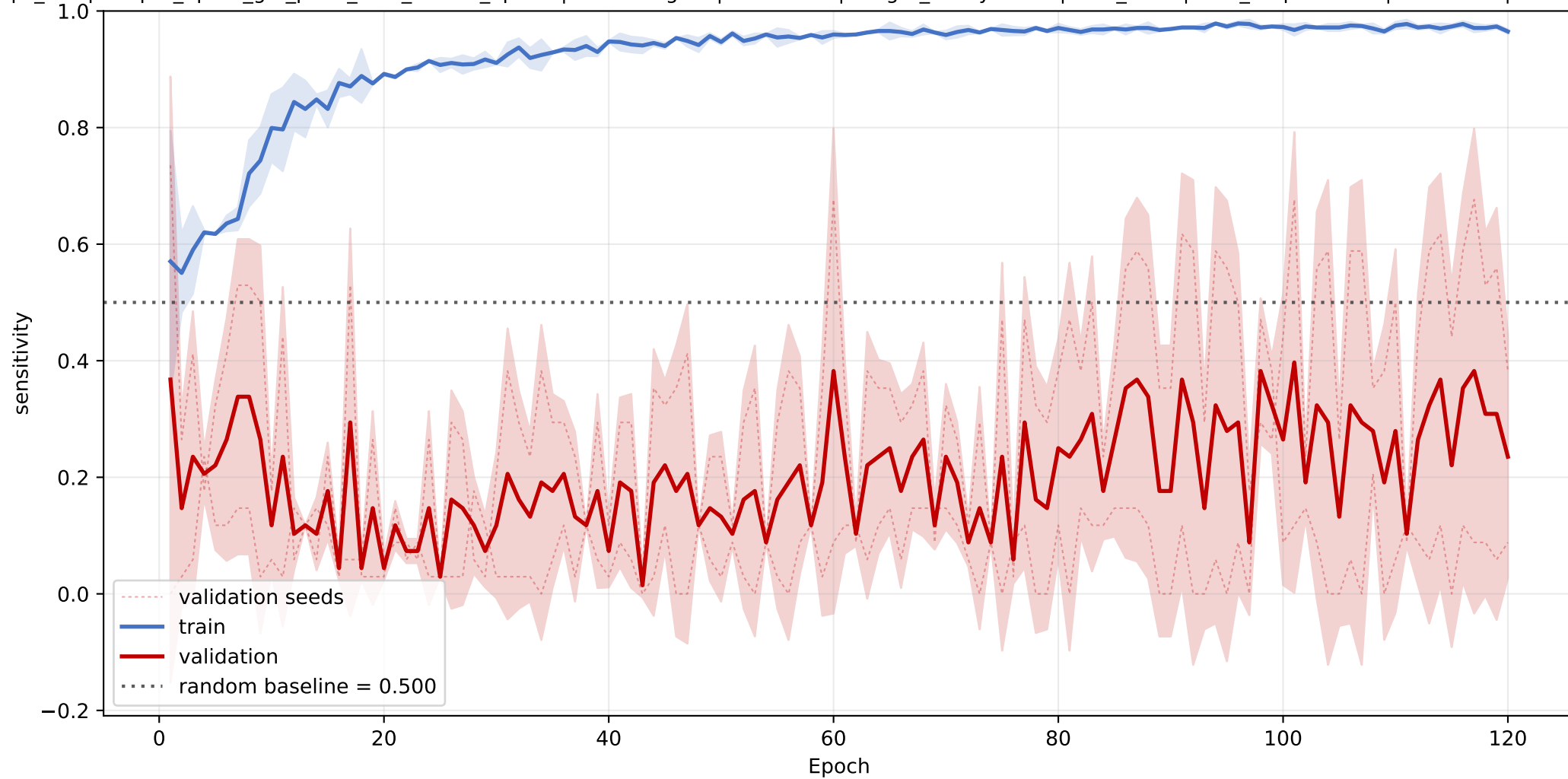
GLTP: mean sensitivity learning curve across seeds
