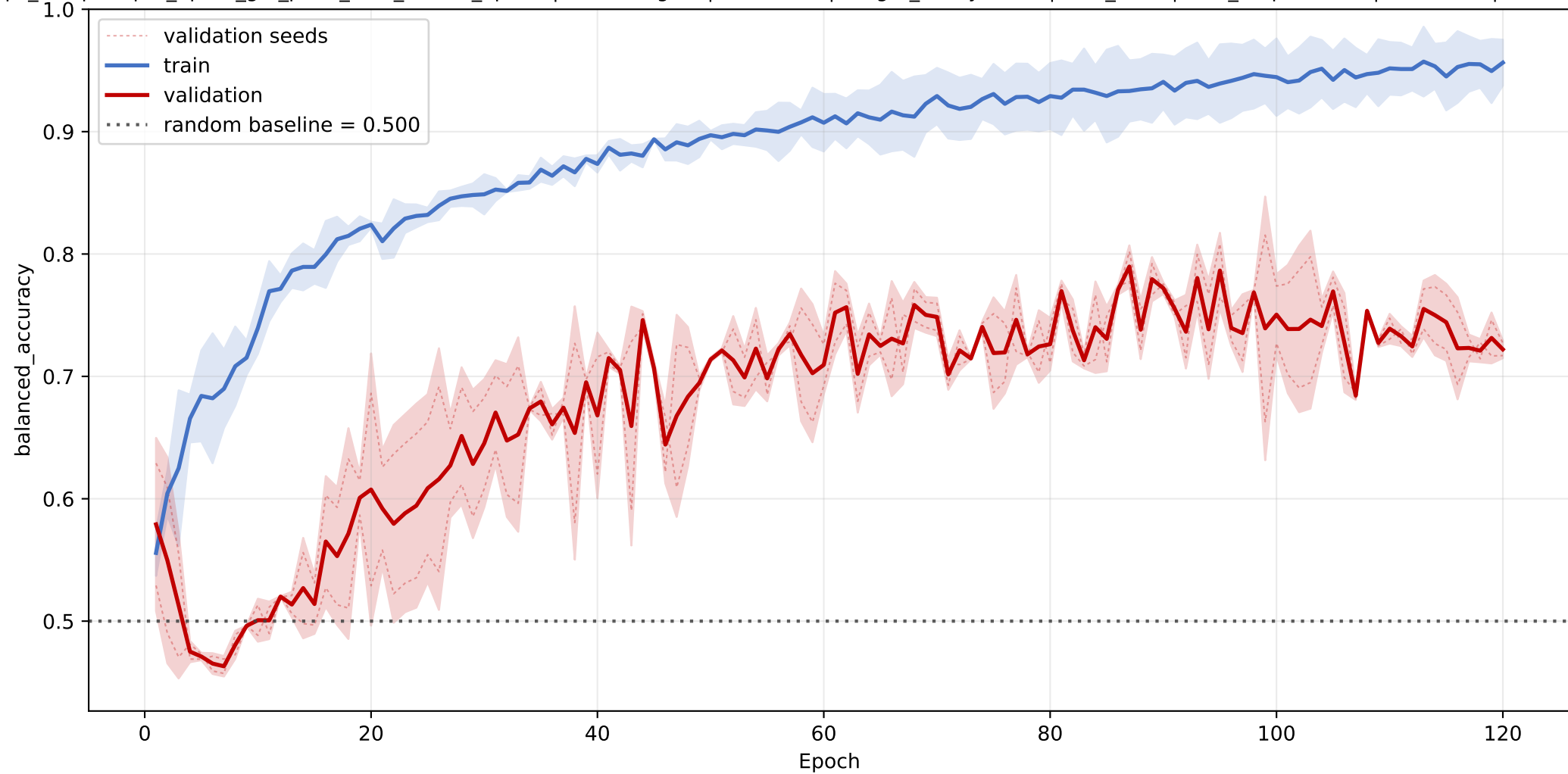
IP_trans: mean balanced accuracy learning curve across seeds
