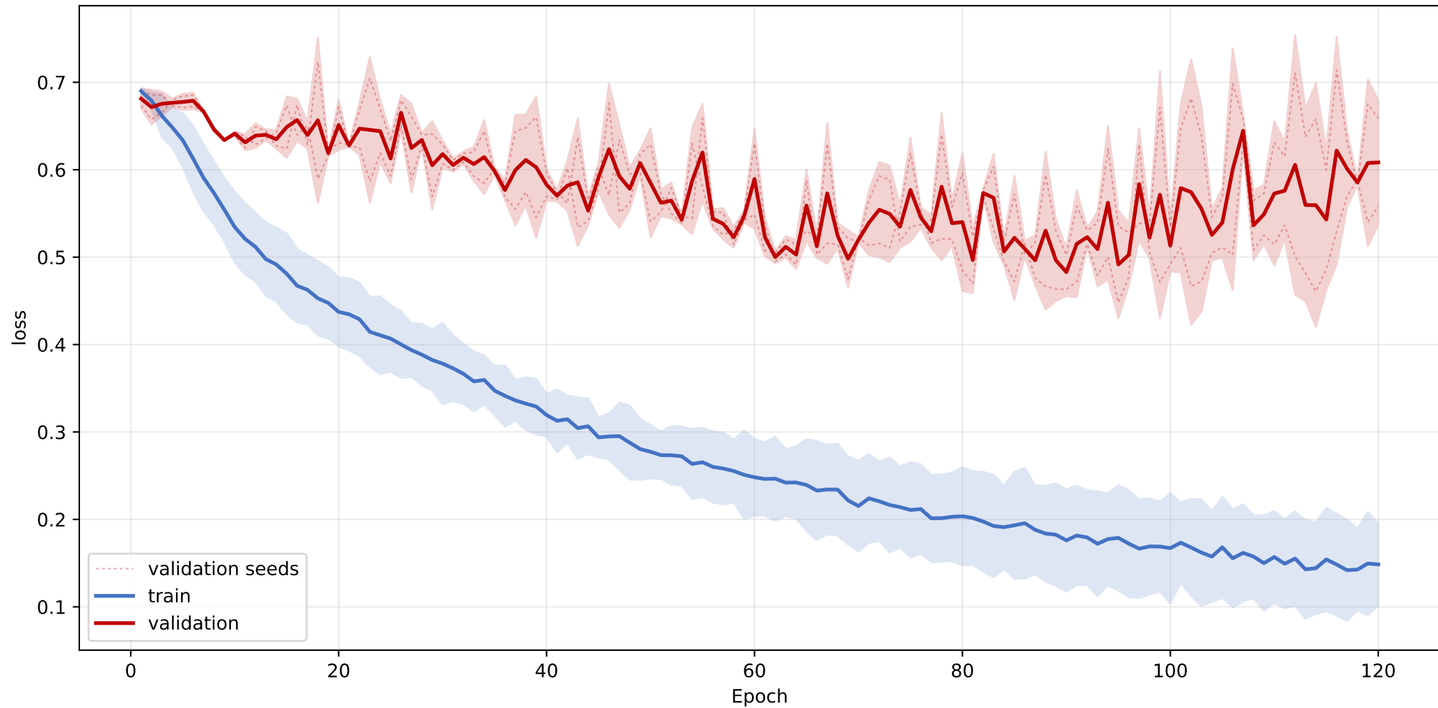
IP_trans: mean loss learning curve across seeds
