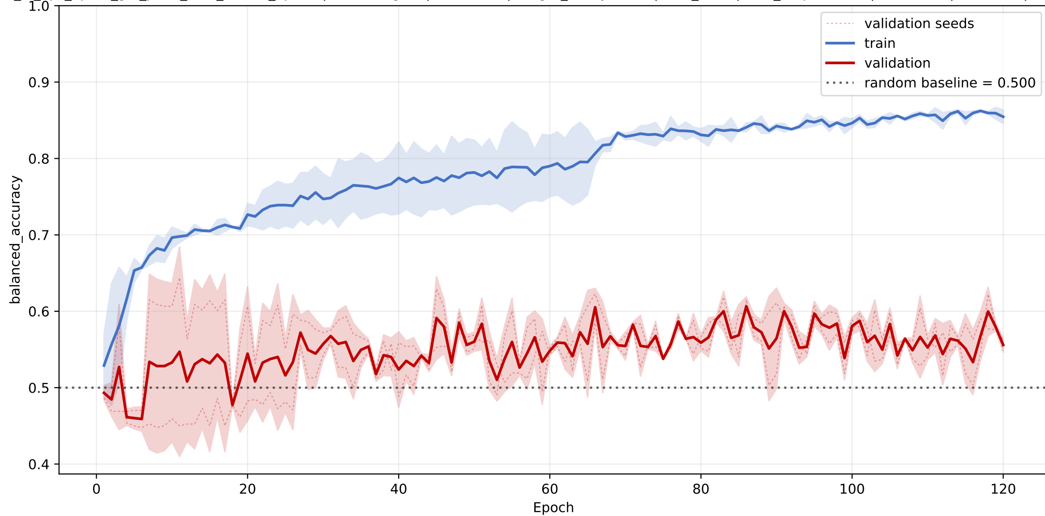
IP_trans: mean balanced_accuracy learning curve across seeds
