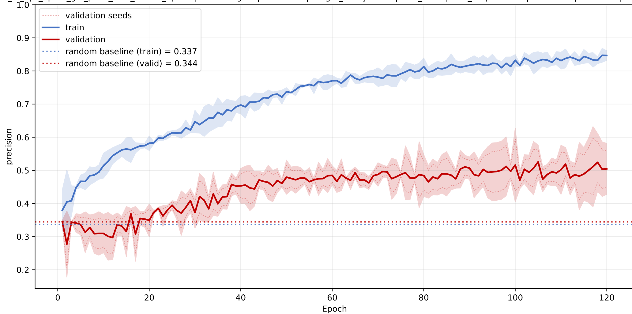
scp2: mean precision learning curve across seeds
