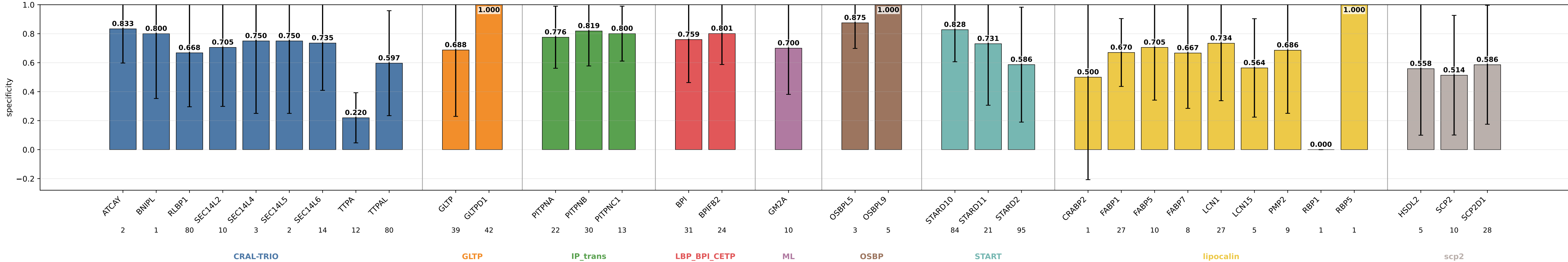
bbp_dcs_smd_fa_nps_dpt01_gm_plm8_hid8_wd001_ep120 specificity by subgroup bbp_dcs_smd_fa_nps_dpt01_gm_plm8_hid8_wd001_ep120 | class weights | lr=0.0001 | weight_decay=0.01 | final_m=4 | final_dropout=0.1 | hiddim=8 | heads=8 | batch=16 | ep=120 | seeds=0,1
