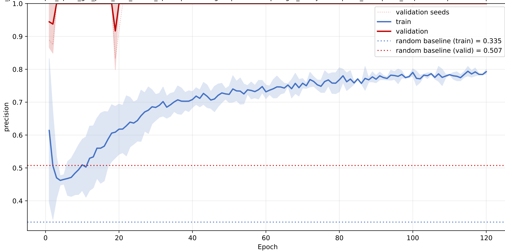
GLTP: mean precision learning curve across seeds
