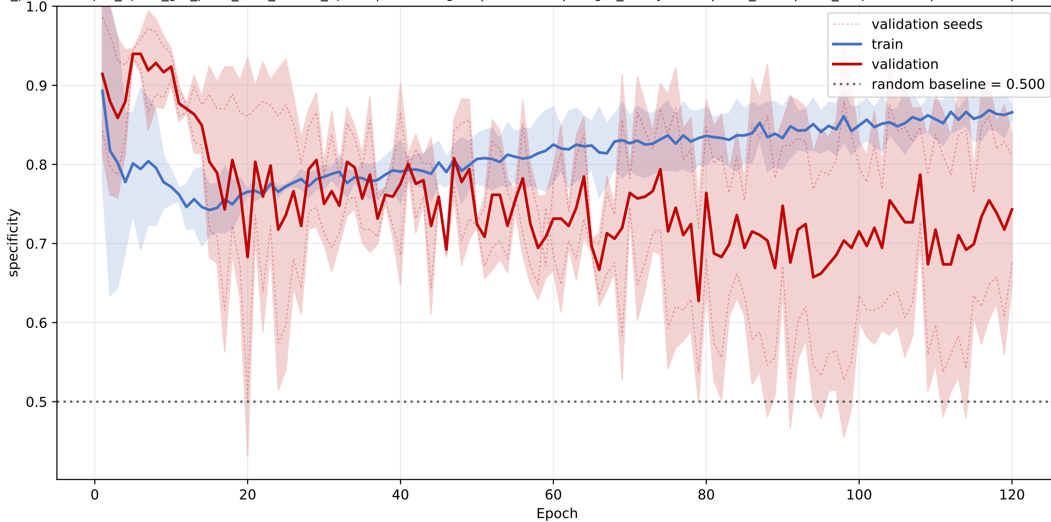
IP_trans: mean specificity learning curve across seeds
