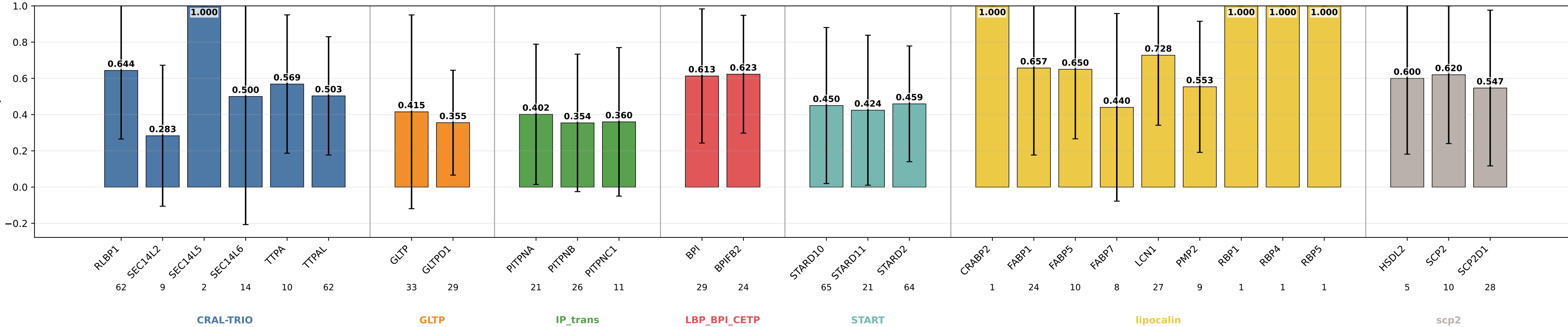
descriptors_2paths sensitivity by subgroup descriptors_2paths | class weights | lr=0.0001 | weight_decay=0.01 | final_m=4 | final_dropout=0.1 | hiddim=8 | heads=8 | batch=16 | ep=120 | seeds=0,1,2,3,4
