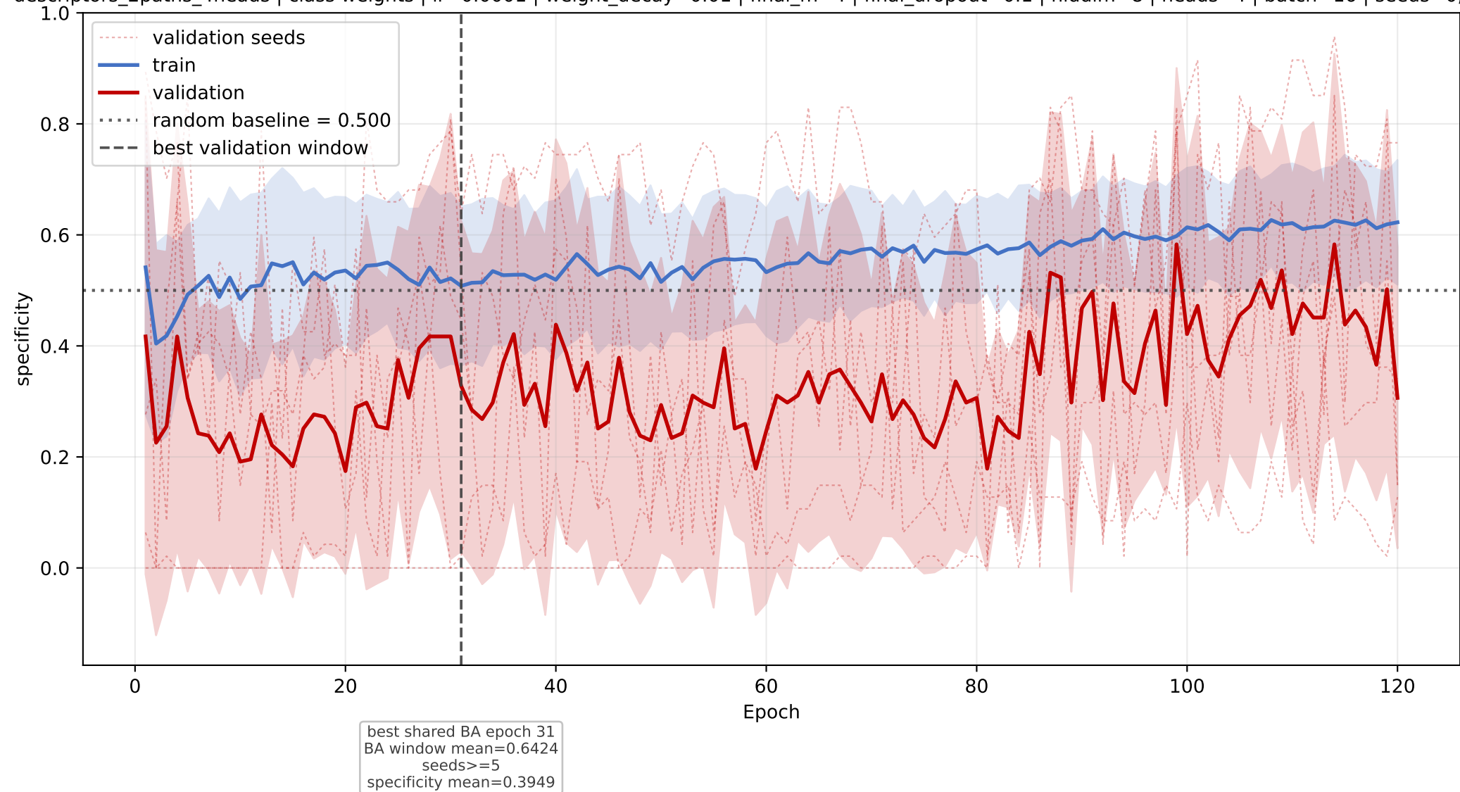
LBP_BPI_CETP: mean specificity learning curve across seeds
