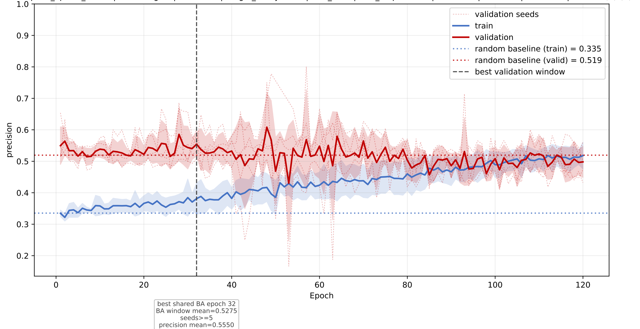
CRAL-TRIO: mean precision learning curve across seeds
