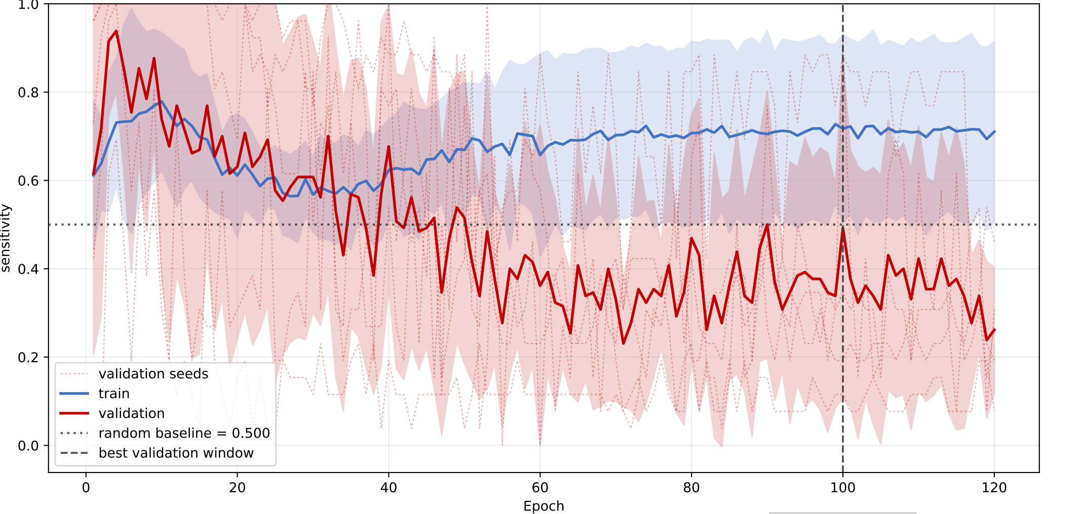
GLTP: mean sensitivity learning curve across seeds
