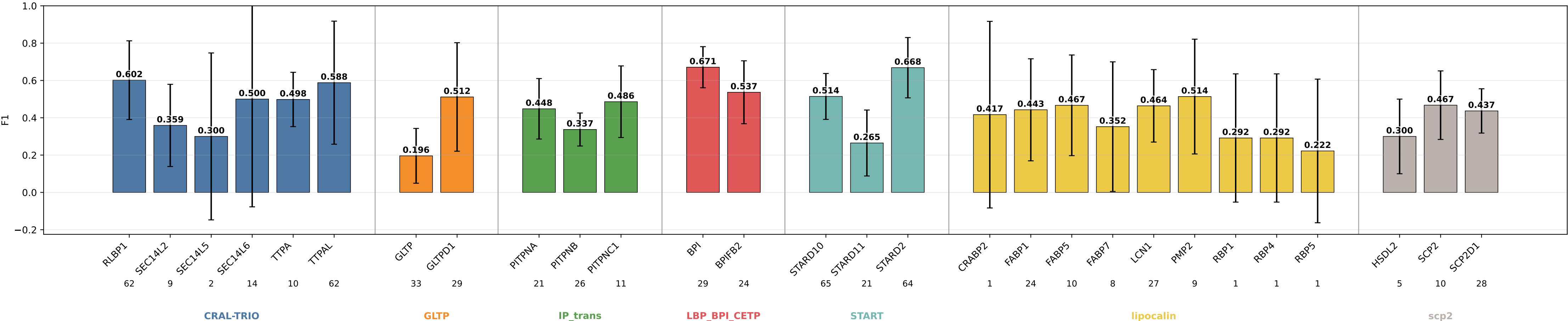
descriptors_2paths_extent F1 by subgroup descriptors_2paths_extent | class weights | lr=0.0001 | weight_decay=0.01 | final_m=4 | final_dropout=0.1 | hiddim=8 | heads=8 | batch=16 | ep=120 | seeds=0,1,2,3,4
