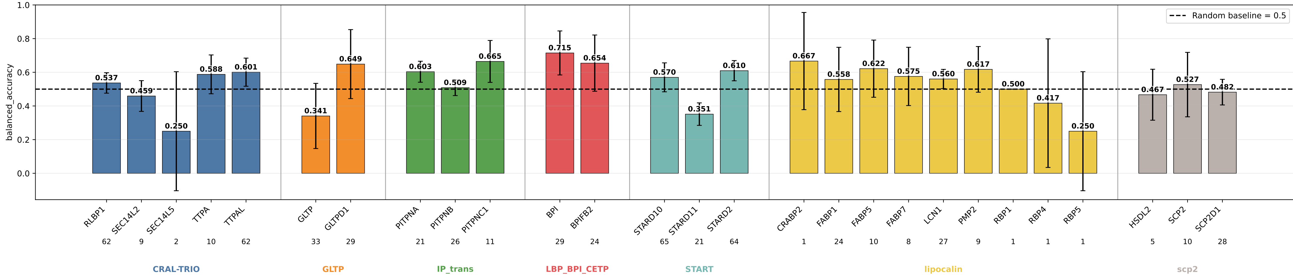
descriptors_2paths_extent balanced_accuracy by subgroup descriptors_2paths_extent | class weights | lr=0.0001 | weight_decay=0.01 | final_m=4 | final_dropout=0.1 | hiddim=8 | heads=8 | batch=16 | ep=120 | seeds=0,1,2,3,4
