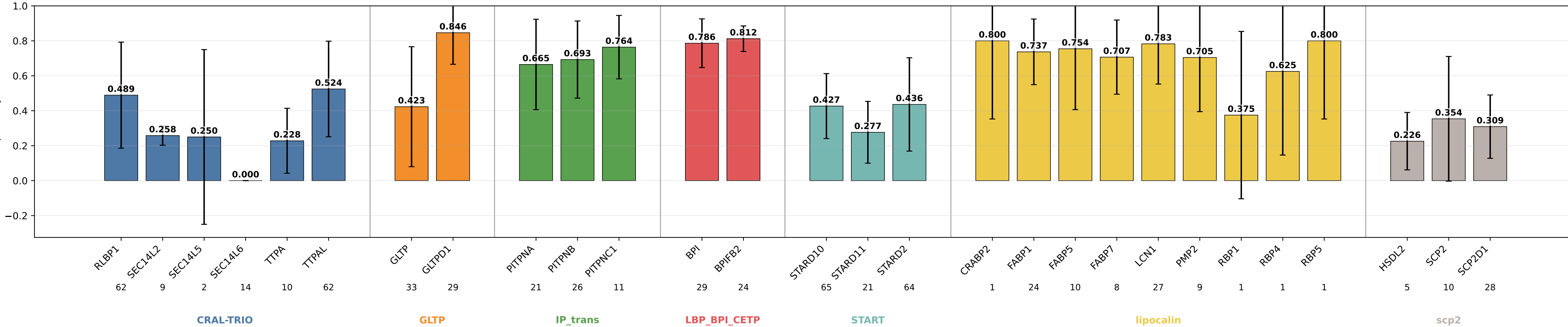
descriptors_2paths_extent_protgeom specificity by subgroup descriptors_2paths_extent_protgeom | class weights | lr=0.0001 | weight_decay=0.01 | final_m=4 | final_dropout=0.1 | hiddim=8 | heads=8 | batch=16 | ep=120 | seeds=0,1,2,3,4
