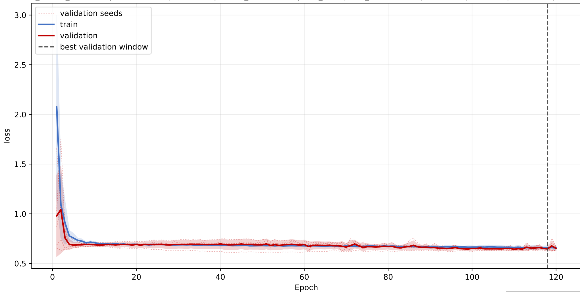
IP_trans: mean loss learning curve across seeds
