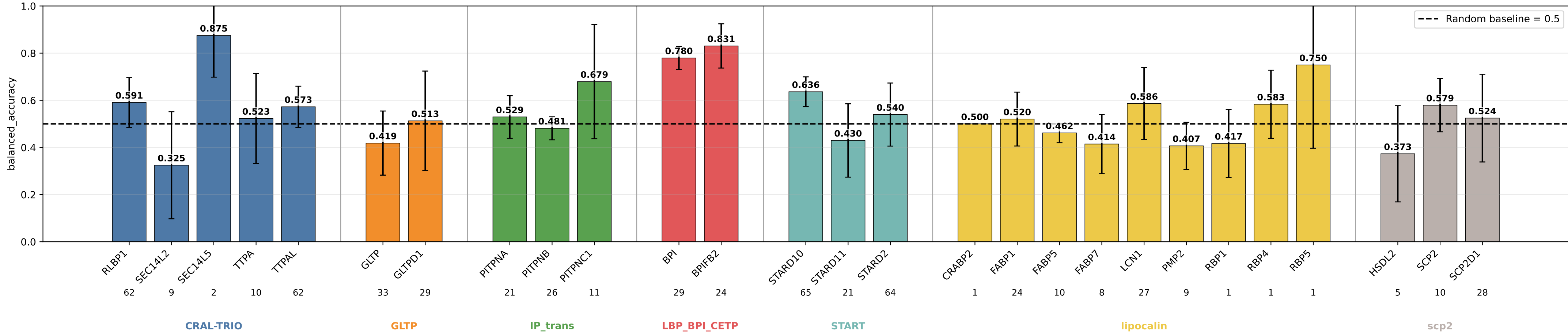
descriptors_2paths_protgeom balanced_accuracy by subgroup descriptors_2paths_protgeom | class weights | lr=0.0001 | weight_decay=0.01 | final_m=4 | final_dropout=0.1 | hiddim=8 | heads=8 | batch=16 | ep=120 | seeds=0,1,2,3,4
