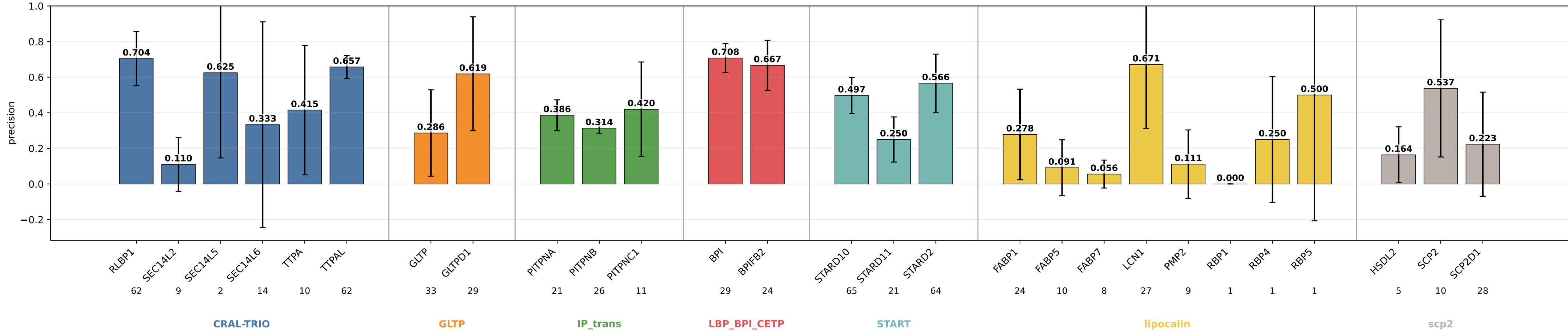
descriptors_2paths_protgeom precision by subgroup descriptors_2paths_protgeom | class weights | lr=0.0001 | weight_decay=0.01 | final_m=4 | final_dropout=0.1 | hiddim=8 | heads=8 | batch=16 | ep=120 | seeds=0,1,2,3,4
