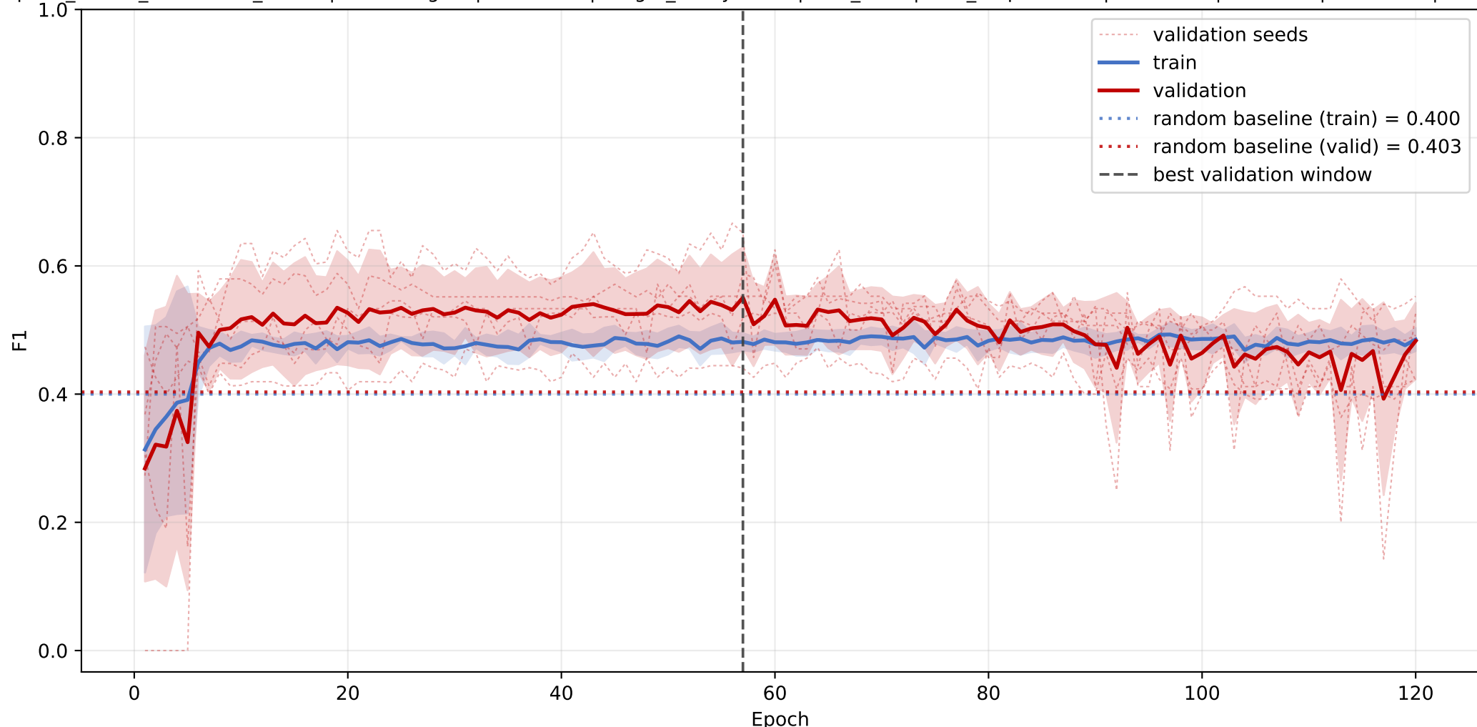
IP_trans: mean F1 learning curve across seeds
