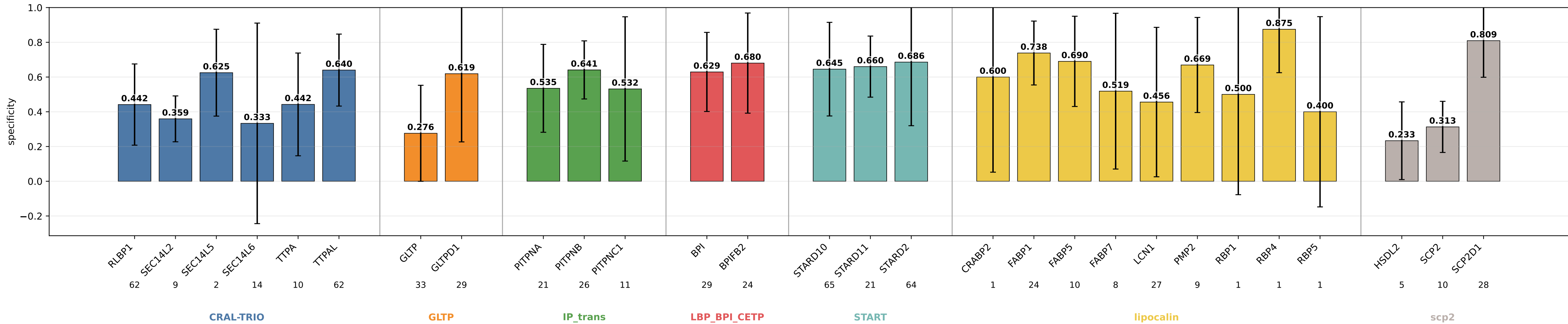
descriptors_coarse_buriedness_match specificity by subgroup descriptors_coarse_buriedness_match | class weights | lr=0.0001 | weight_decay=0.01 | final_m=4 | final_dropout=0.1 | hiddim=8 | heads=8 | batch=16 | ep=120 | seeds=0,1,2,3,4
