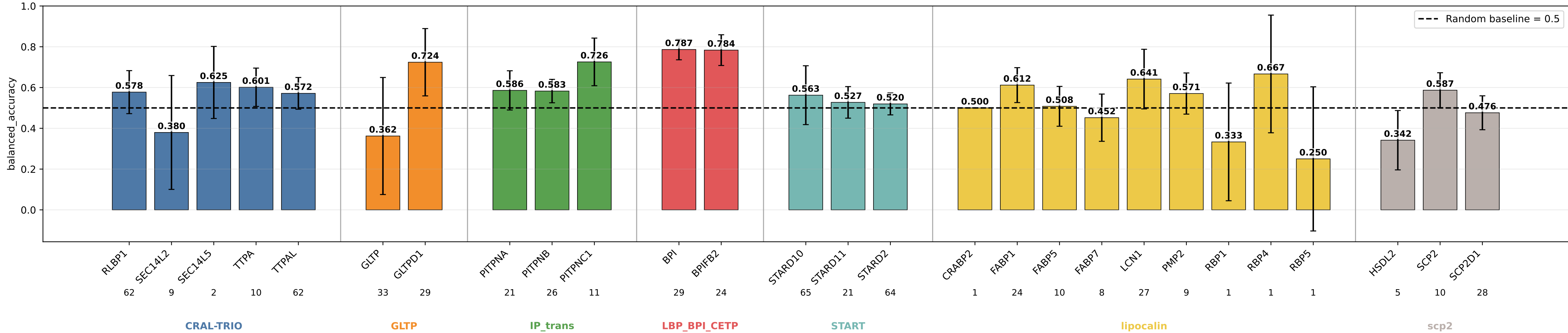
descriptors_coarse_hydrocore balanced_accuracy by subgroup descriptors_coarse_hydrocore | class weights | lr=0.0001 | weight_decay=0.01 | final_m=4 | final_dropout=0.1 | hiddim=8 | heads=8 | batch=16 | ep=120 | seeds=0,1,2,3,4
