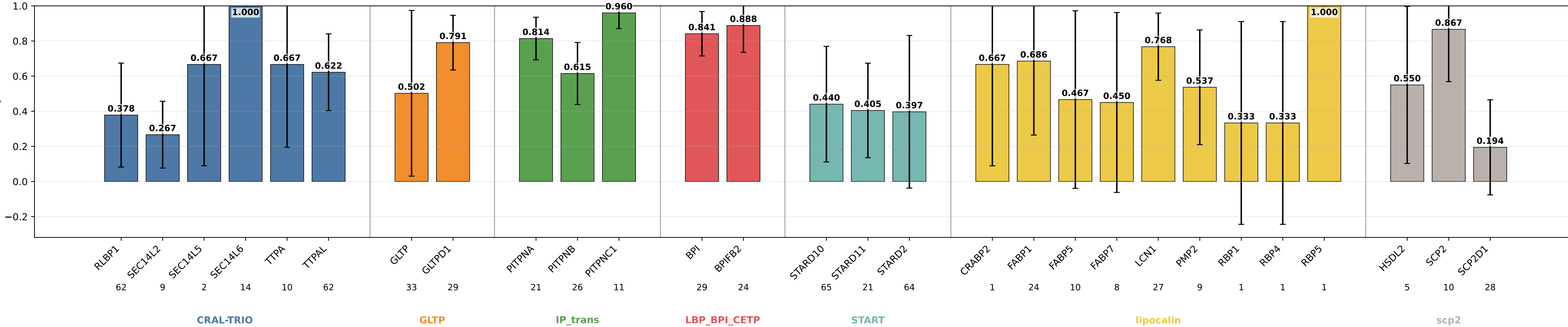
descriptors_coarse_pocket_elongation sensitivity by subgroup descriptors_coarse_pocket_elongation | class weights | lr=0.0001 | weight_decay=0.01 | final_m=4 | final_dropout=0.1 | hiddim=8 | heads=8 | batch=16 | ep=120 | seeds=0,1,2,3,4
