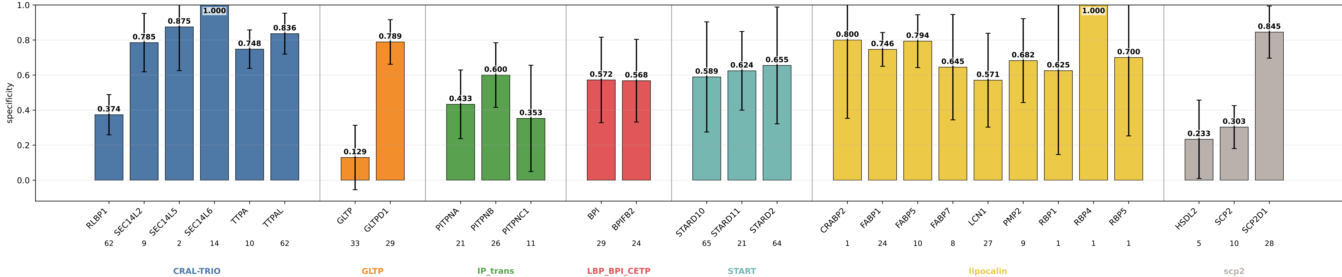
descriptors_coarse_tail_elongation_fit specificity by subgroup descriptors_coarse_tail_elongation_fit | class weights | lr=0.0001 | weight_decay=0.01 | final_m=4 | final_dropout=0.1 | hiddim=8 | heads=8 | batch=16 | ep=120 | seeds=0,1,2,3,4
