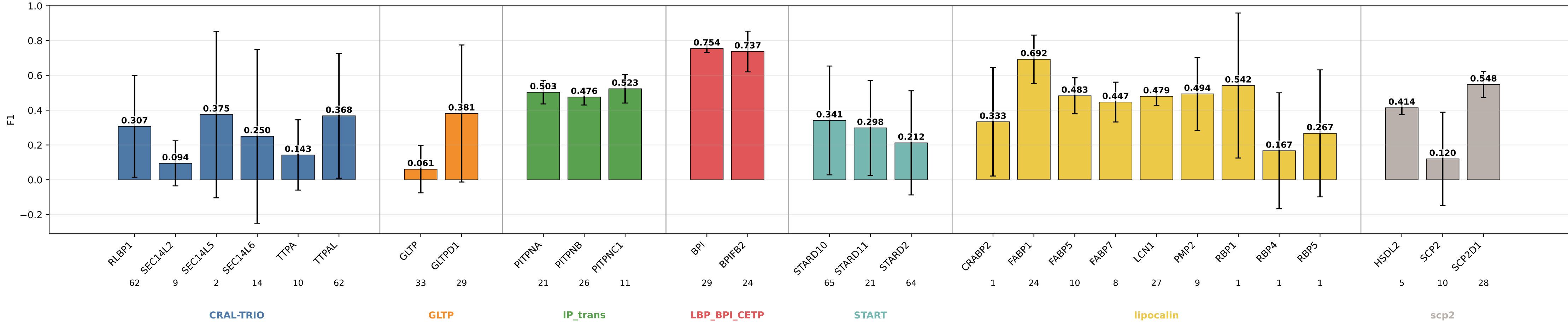
descriptors_path_v2 F1 by subgroup descriptors_path_v2 | class weights | lr=0.0001 | weight_decay=0.01 | final_m=4 | final_dropout=0.1 | hiddim=8 | heads=8 | batch=16 | ep=120 | seeds=0,1,2,3,4
