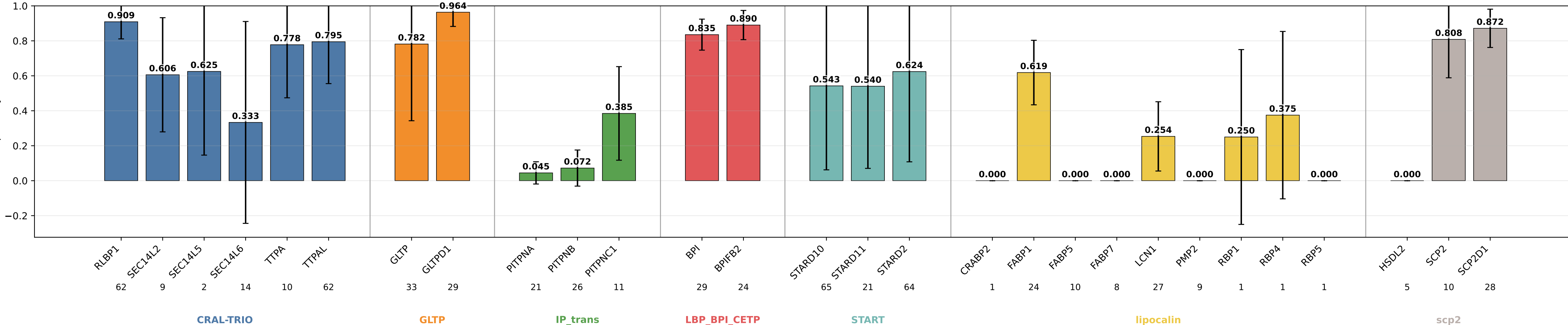
descriptors_path_v2 specificity by subgroup descriptors_path_v2 | class weights | lr=0.0001 | weight_decay=0.01 | final_m=4 | final_dropout=0.1 | hiddim=8 | heads=8 | batch=16 | ep=120 | seeds=0,1,2,3,4
