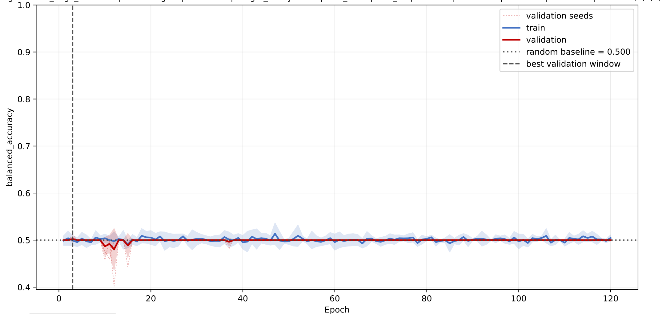
CRAL-TRIO: mean balanced_accuracy learning curve across seeds
