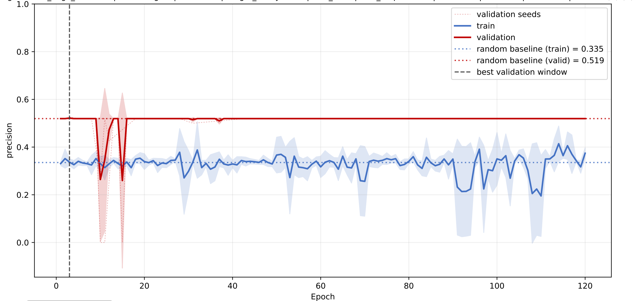
CRAL-TRIO: mean precision learning curve across seeds
