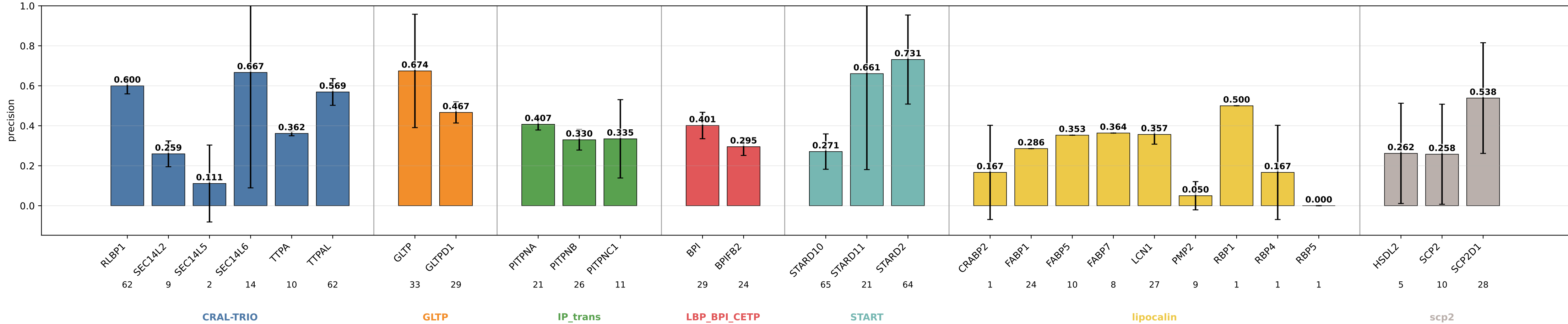
geometric_edge_attention precision by subgroup geometric_edge_attention | class weights | lr=0.0001 | weight_decay=0.01 | final_m=4 | final_dropout=0.1 | hiddim=8 | heads=8 | batch=16 | ep=120 | seeds=0,1,2,3,4
