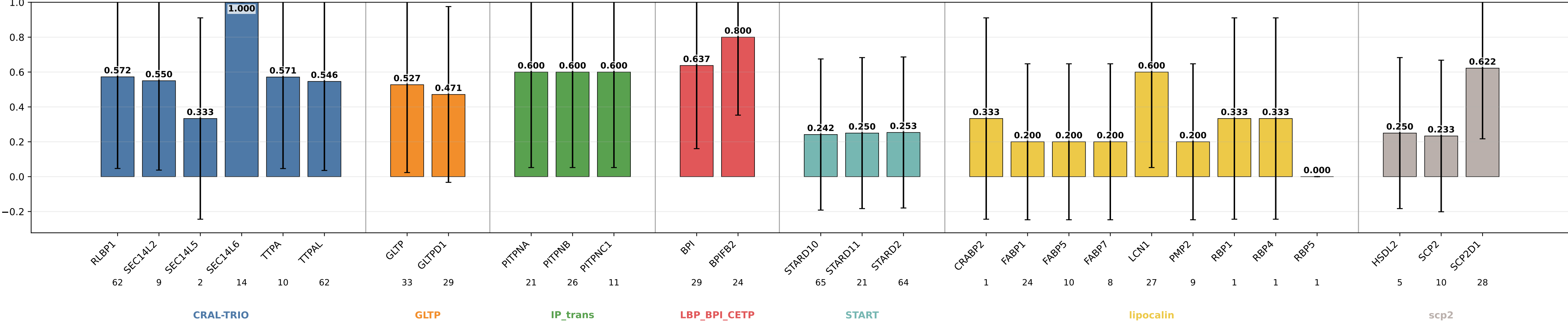
geometric_edge_attention sensitivity by subgroup geometric_edge_attention | class weights | lr=0.0001 | weight_decay=0.01 | final_m=4 | final_dropout=0.1 | hiddim=8 | heads=8 | batch=16 | ep=120 | seeds=0,1,2,3,4
