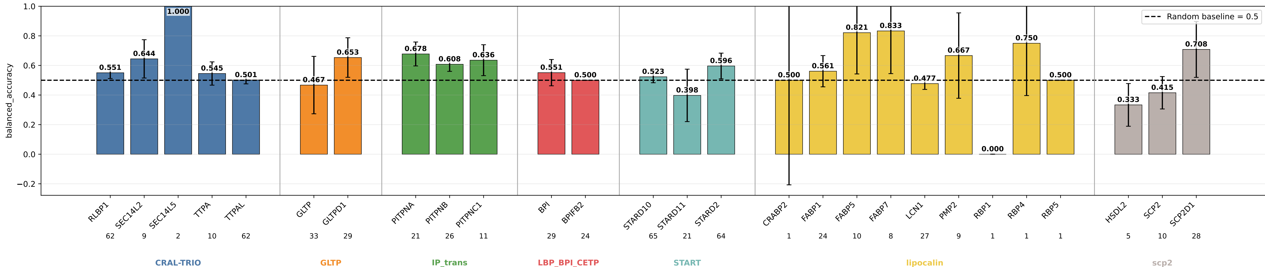
geometric_edge_attention_add_nwd balanced_accuracy by subgroup geometric_edge_attention_add_nwd | class weights | lr=0.0001 | weight_decay=1e-05 | final_m=4 | final_dropout=0.1 | hiddim=8 | heads=8 | batch=16 | ep=120 | seeds=0,1,2
