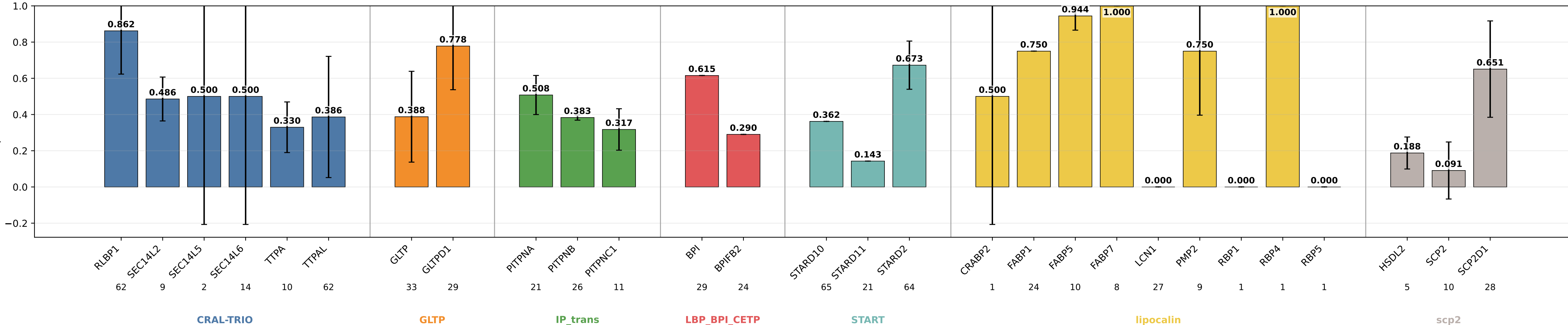
geometric_edge_attention_add_nwd precision by subgroup geometric_edge_attention_add_nwd | class weights | lr=0.0001 | weight_decay=1e-05 | final_m=4 | final_dropout=0.1 | hiddim=8 | heads=8 | batch=16 | ep=120 | seeds=0,1,2
