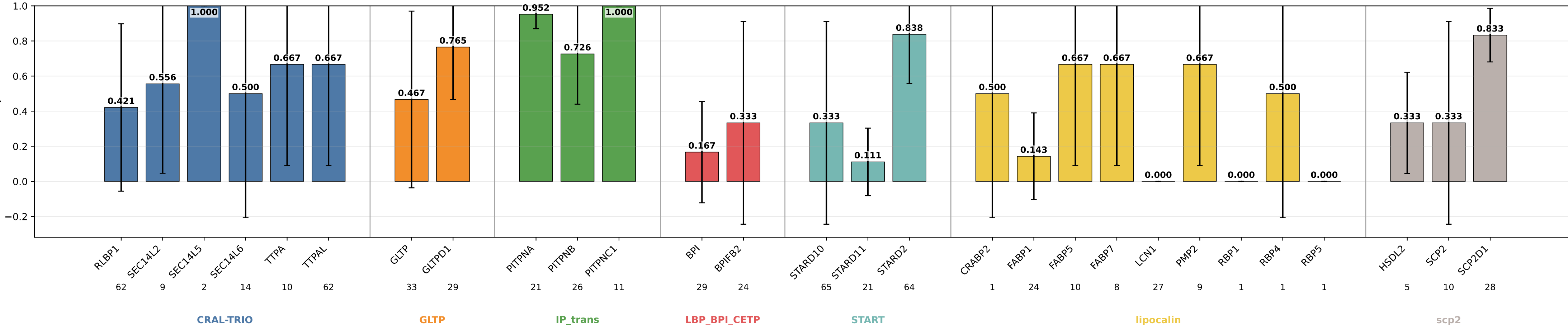
geometric_edge_attention_add_nwd sensitivity by subgroup geometric_edge_attention_add_nwd | class weights | lr=0.0001 | weight_decay=1e-05 | final_m=4 | final_dropout=0.1 | hiddim=8 | heads=8 | batch=16 | ep=120 | seeds=0,1,2
