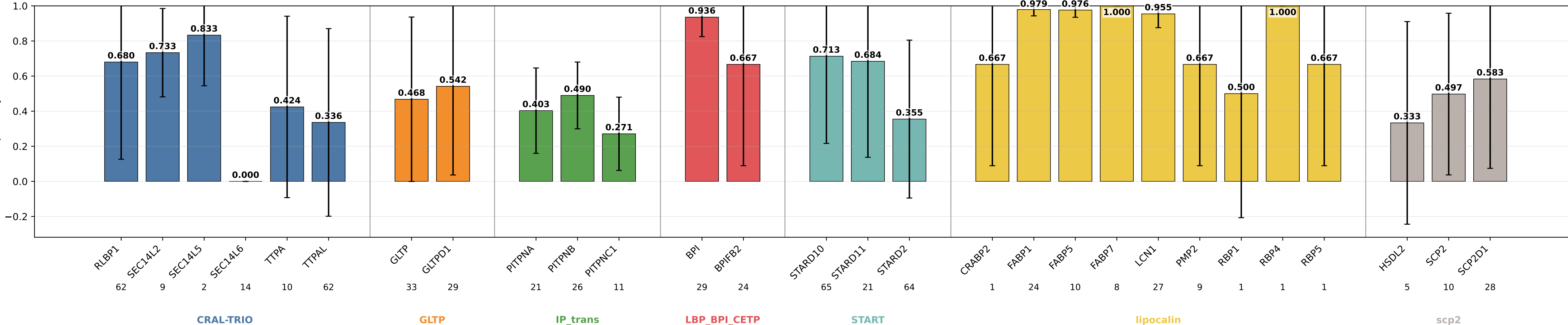
geometric_edge_attention_add_nwd specificity by subgroup geometric_edge_attention_add_nwd | class weights | lr=0.0001 | weight_decay=1e-05 | final_m=4 | final_dropout=0.1 | hiddim=8 | heads=8 | batch=16 | ep=120 | seeds=0,1,2
