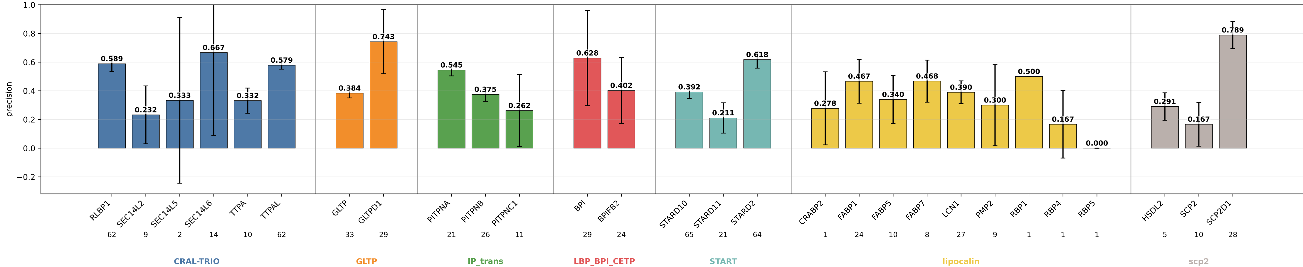
geometric_edge_attention_add_nwd_hid16 precision by subgroup geometric_edge_attention_add_nwd_hid16 | class weights | lr=0.0001 | weight_decay=1e-05 | final_m=4 | final_dropout=0.1 | hiddim=16 | heads=8 | batch=16 | ep=120 | seeds=0,1,2
