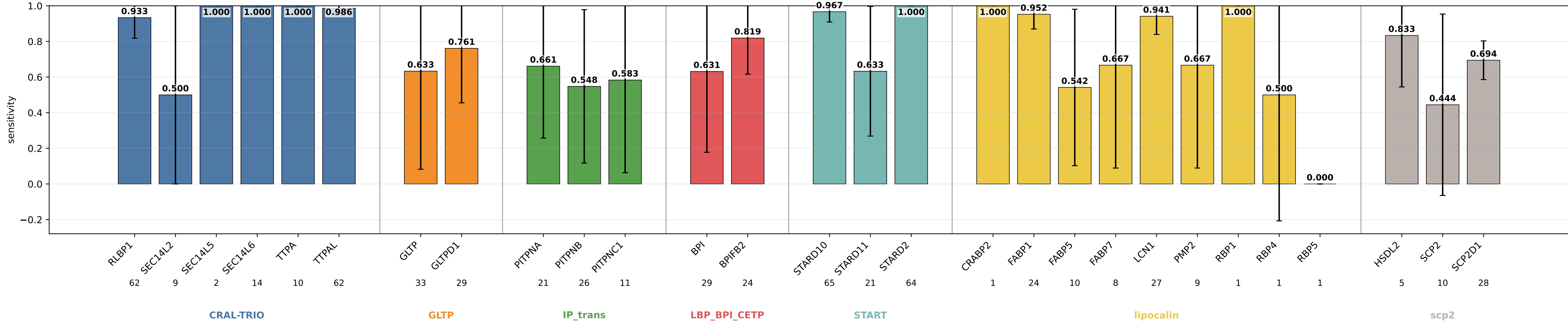
geometric_edge_attention_add_nwd_hid16 sensitivity by subgroup geometric_edge_attention_add_nwd_hid16 | class weights | lr=0.0001 | weight_decay=1e-05 | final_m=4 | final_dropout=0.1 | hiddim=16 | heads=8 | batch=16 | ep=120 | seeds=0,1,2
