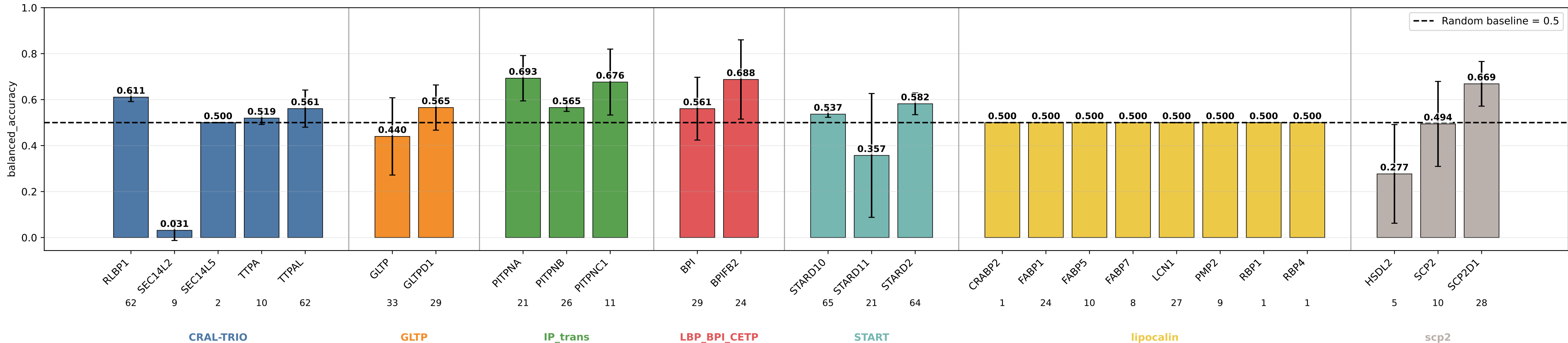
geometric_edge_attention_nwd balanced_accuracy by subgroup geometric_edge_attention_nwd | class weights | lr=0.0001 | weight_decay=1e-05 | final_m=4 | final_dropout=0.1 | hiddim=8 | heads=8 | batch=16 | ep=120 | seeds=0,1
