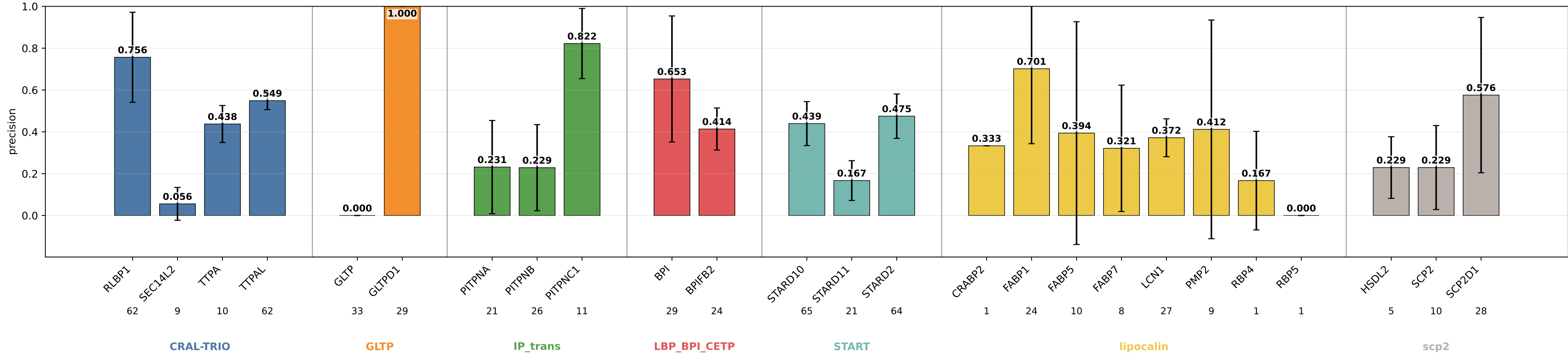
geometric_edge_attention_nwd_no_lipid_graphs precision by subgroup geometric_edge_attention_nwd_no_lipid_graphs | class weights | lr=0.0001 | weight_decay=1e-05 | final_m=4 | final_dropout=0.1 | hiddim=8 | heads=8 | batch=16 | ep=120 | seeds=0,1,2
