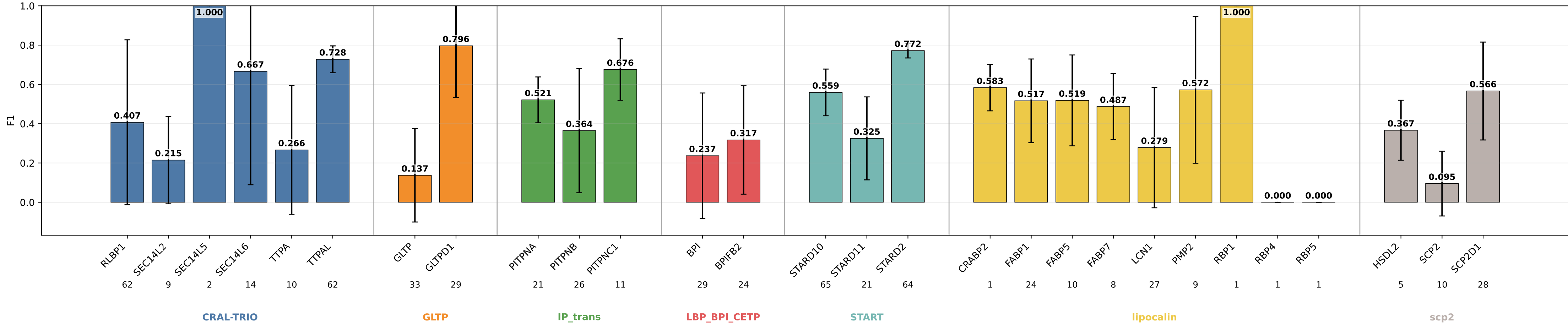
geometric_edge_attention_protgeom8 F1 by subgroup geometric_edge_attention_protgeom8 | class weights | lr=0.0001 | weight_decay=0.01 | final_m=4 | final_dropout=0.1 | hiddim=8 | heads=8 | batch=16 | ep=120 | seeds=0,1,2
